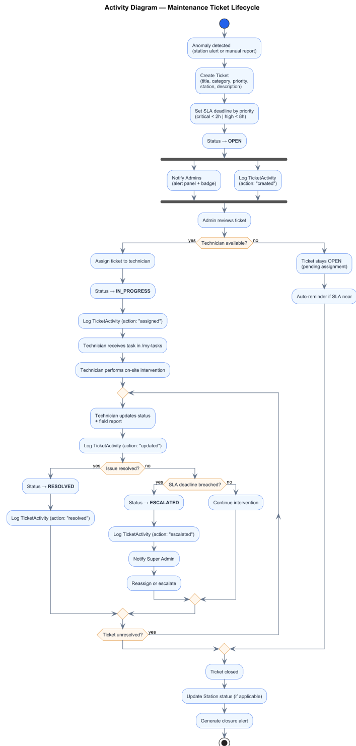
Figure 3.4: Activity Diagram — Maintenance Ticket Lifecycle
