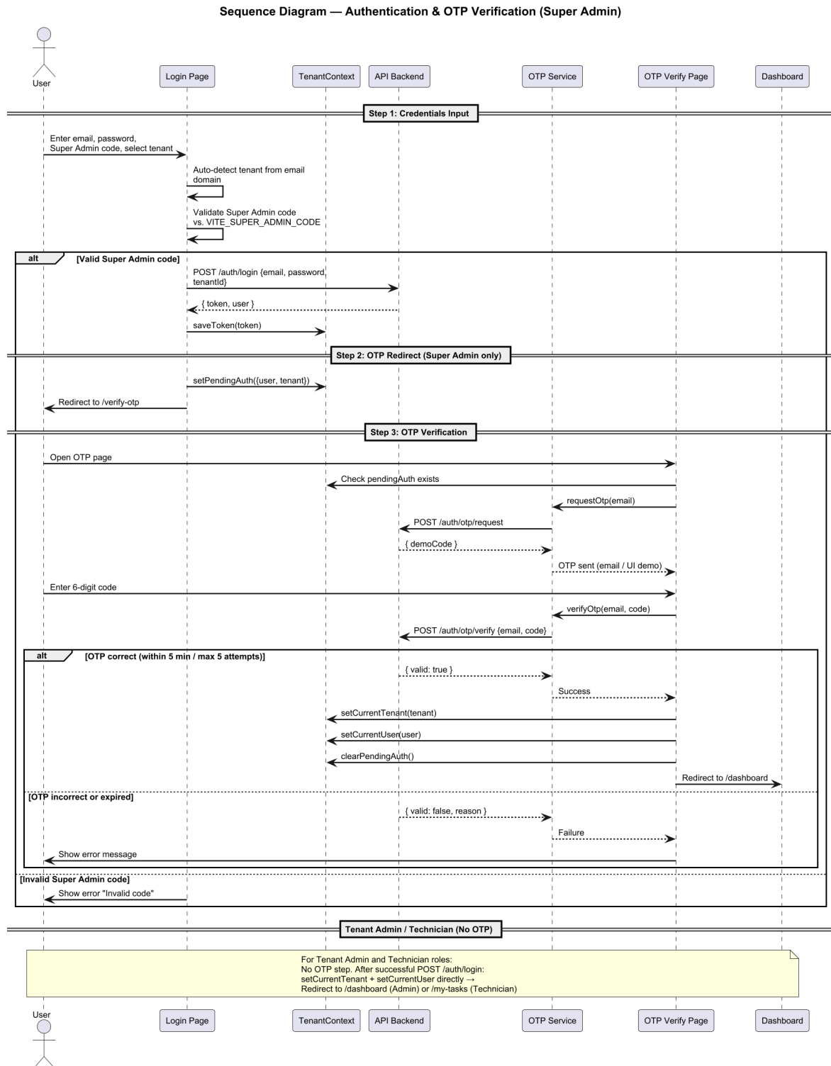
Figure 3.3: Sequence Diagram — Authentication and OTP Verification Flow (Super Admin)
